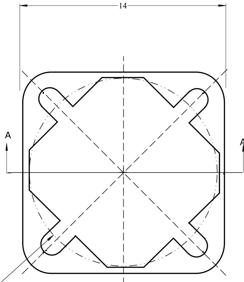
BOTTOM VIEW
