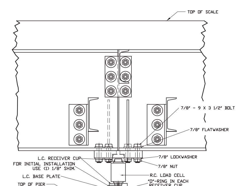
VIEW B-B
