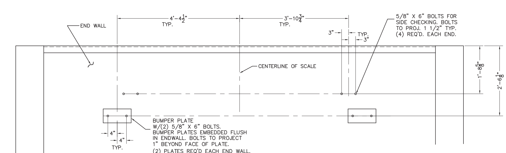
END WALL CHECKING DETAIL
