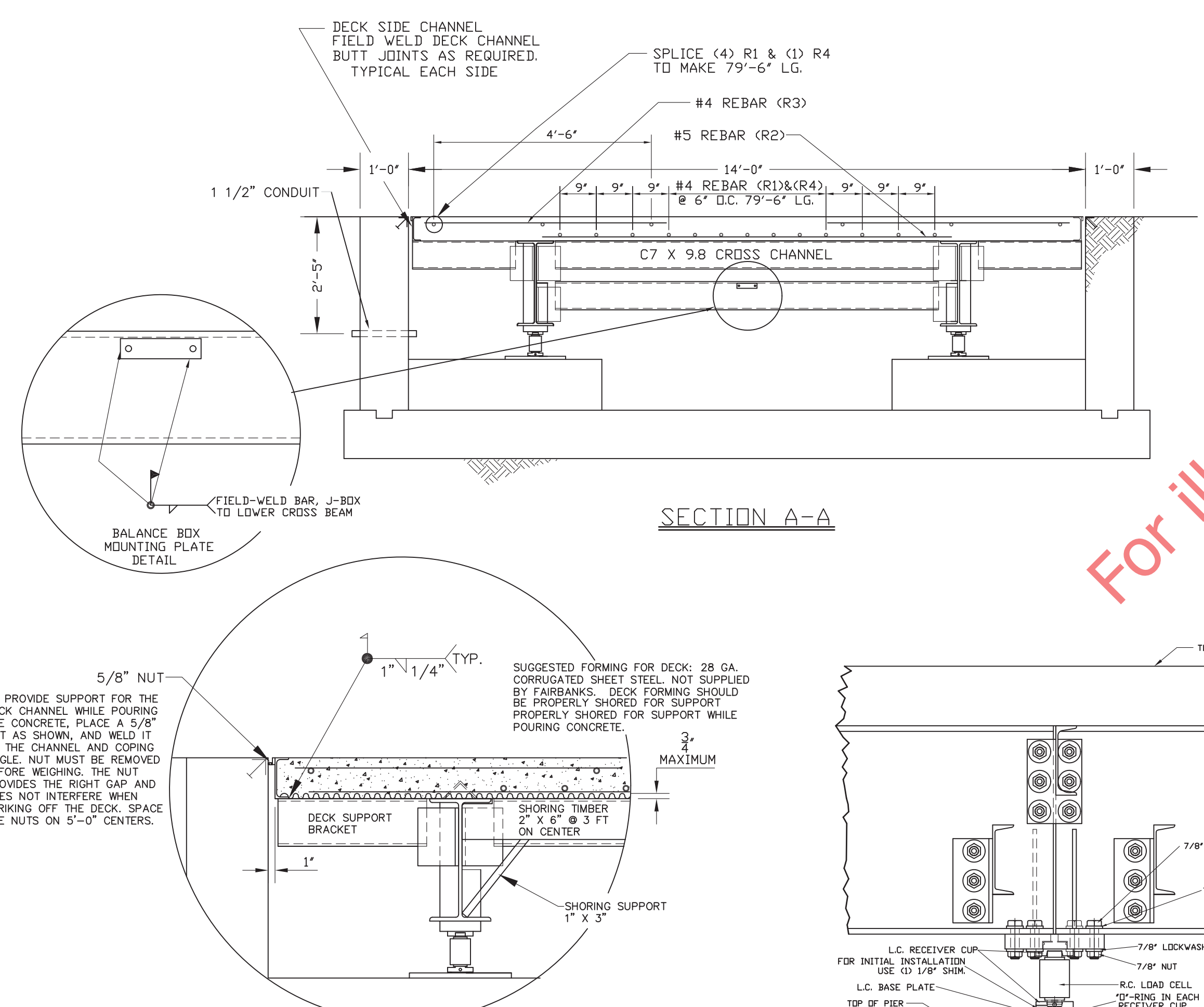
DECK FORMING DETAIL
