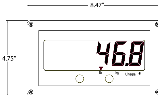
Panel mount remote display
